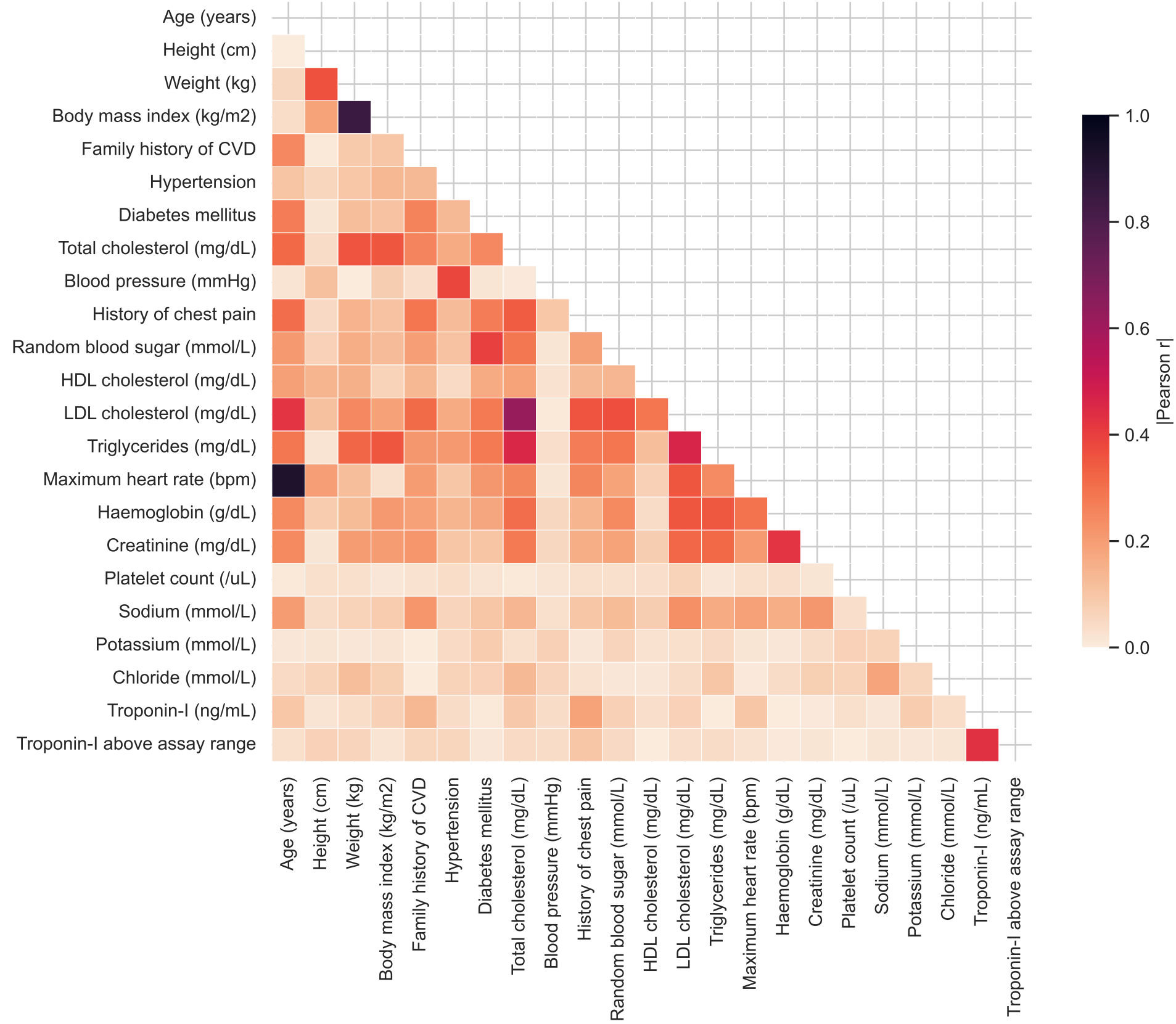
Figure 4. Absolute pairwise correlation between numeric predictors (training partition)
